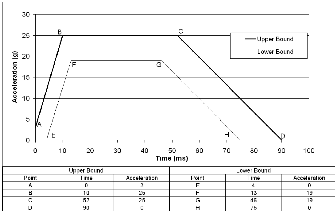
Figure 2 — Test Platform Acceleration Graph
