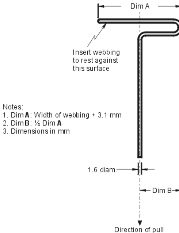
Figure 3 — Webbing Tension Pull Device
