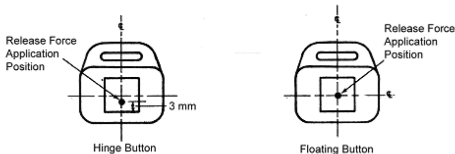
Figure 1(b) — Release Force Application Position for Push-Button Mechanisms
