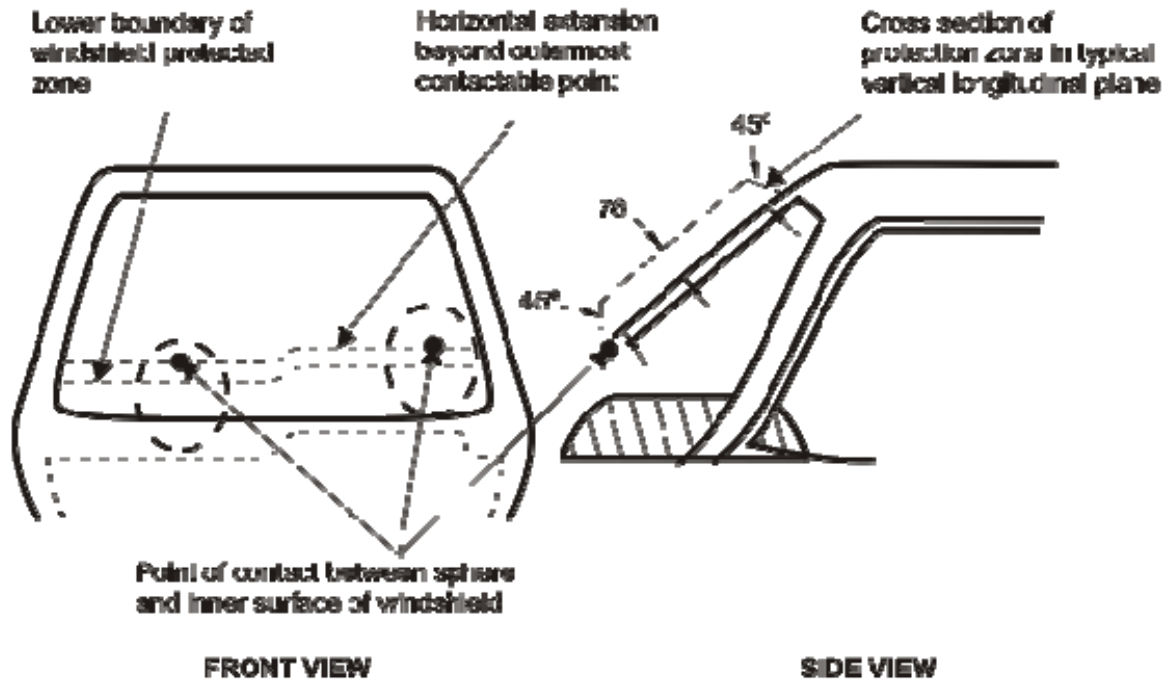
Figure 1 - Windshield Protection Zone
