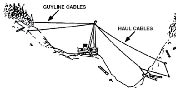
Figure 2.1 – Highlead Spar
