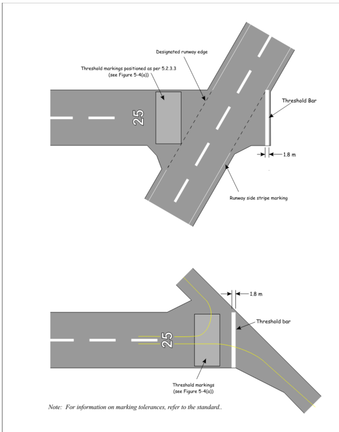
Figure 5-4(b): Threshold markings (with threshold bar)
