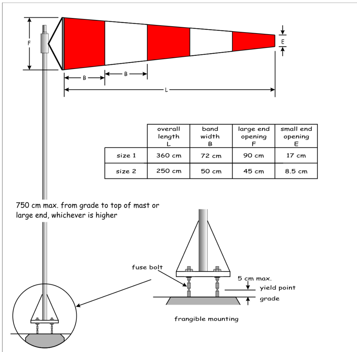
Figure 5-1: Typical wind direction indicator
