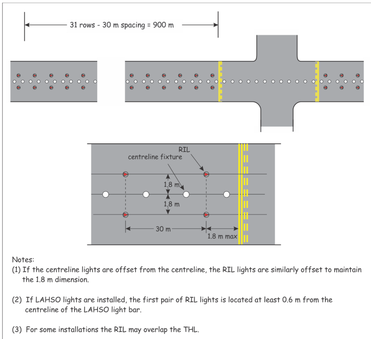
Figure 5-46: Runway status lights—runway intersection lights (RIL)
