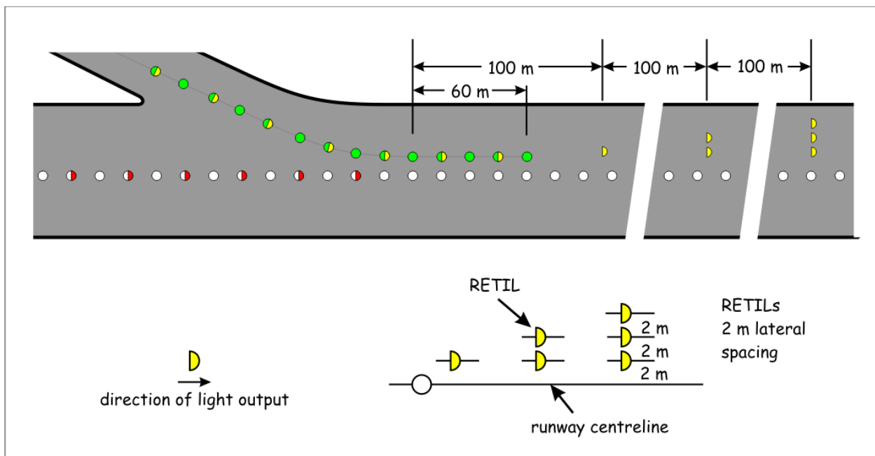
Figure 5-48: Rapid exit taxiway indicator lights (RETIL)
