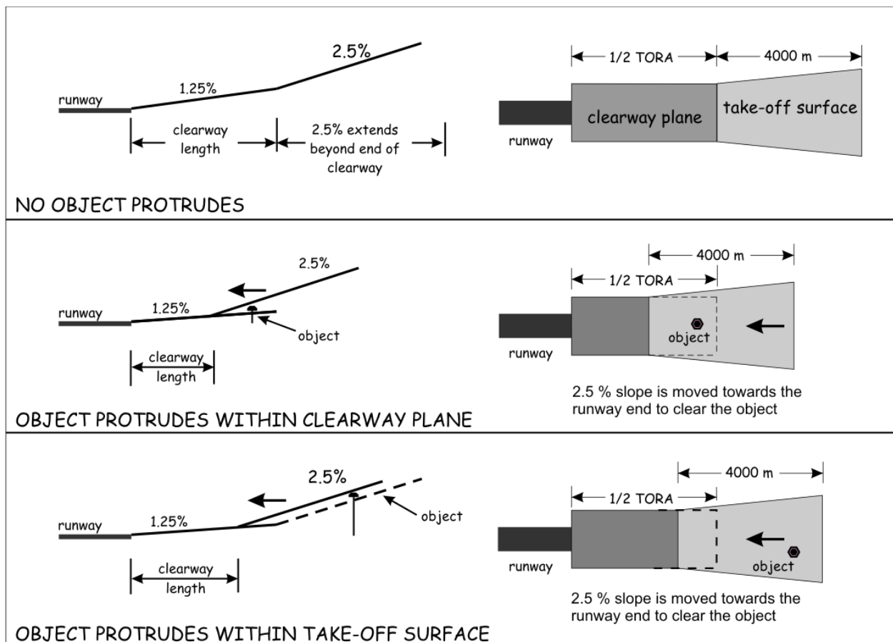
Figure 4-9: Clearway plane
