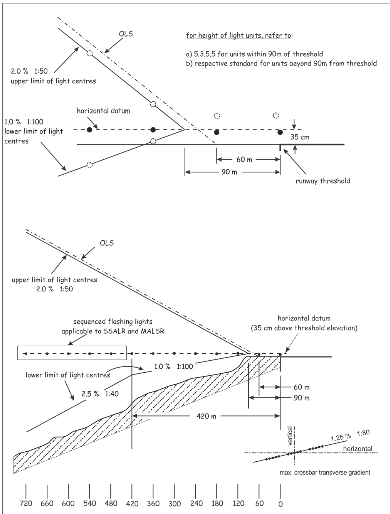
Figure 5-27: SSALR / SSALS / MALSR / MALSF / MALS profile and limit of light centres
