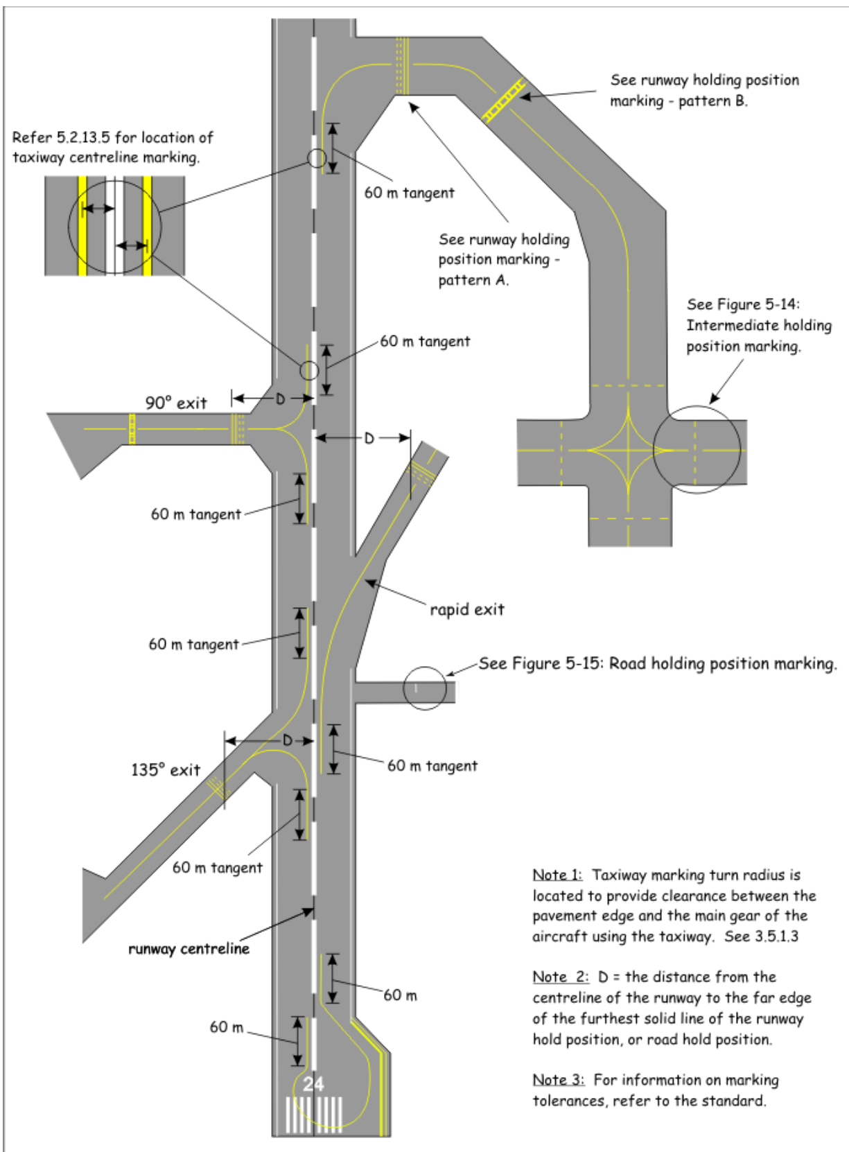
Figure 5-8: Taxiway markings
