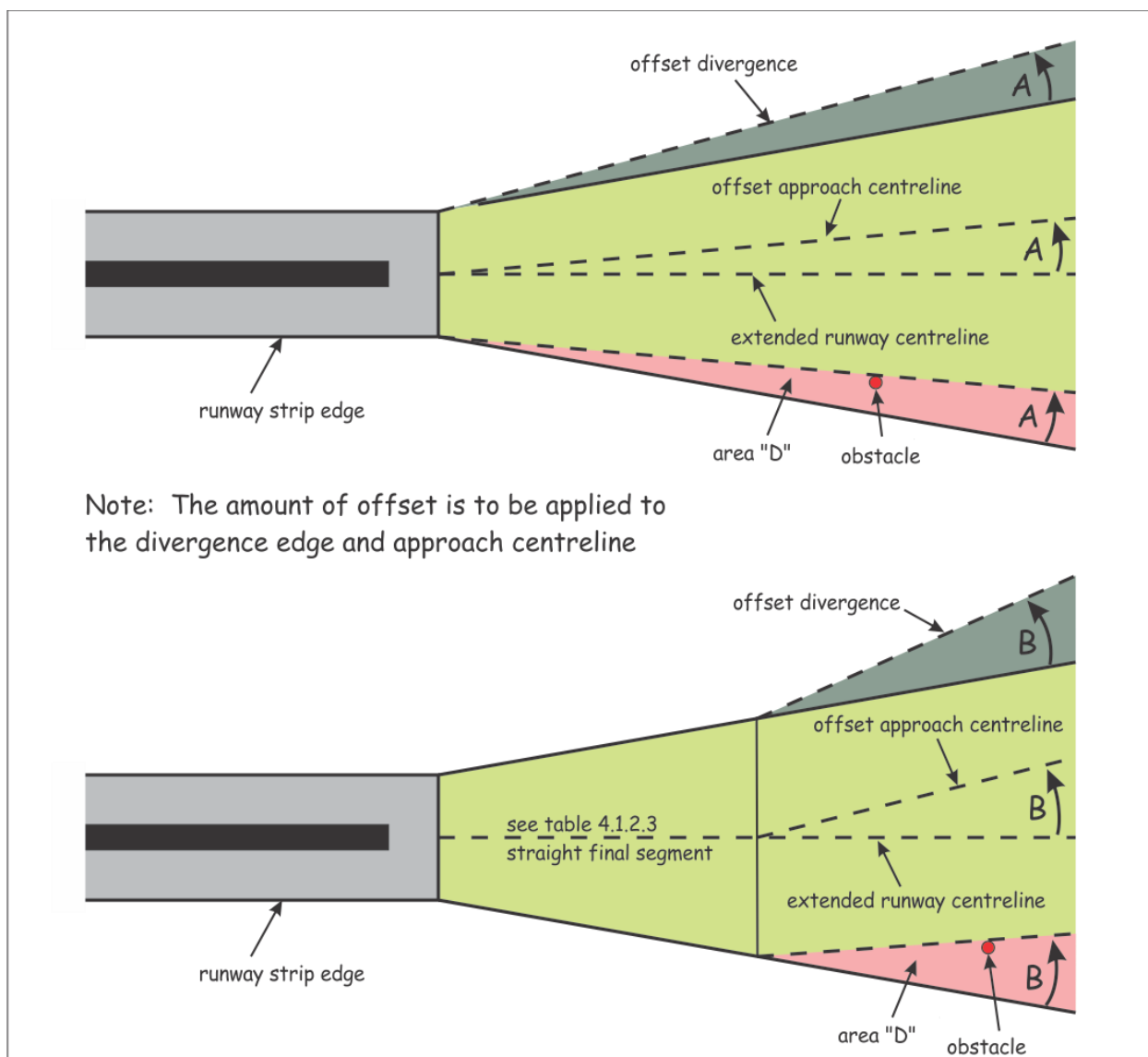
Figure 4-3(b): Offset approach surface (Non-instrument runways)
