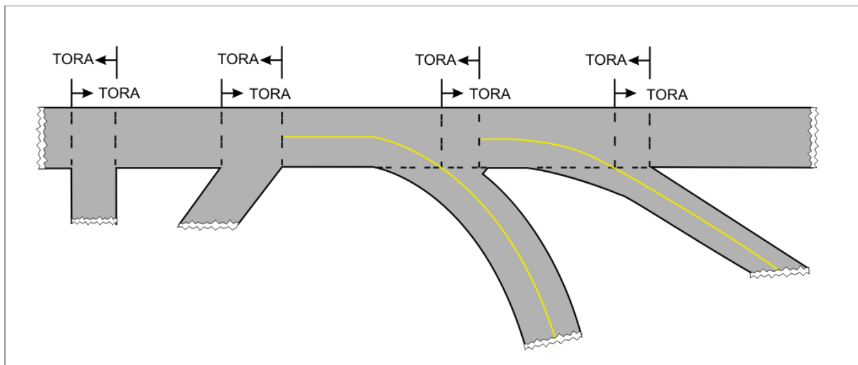
Figure 2-3: Illustration of intersection take-off run distances
