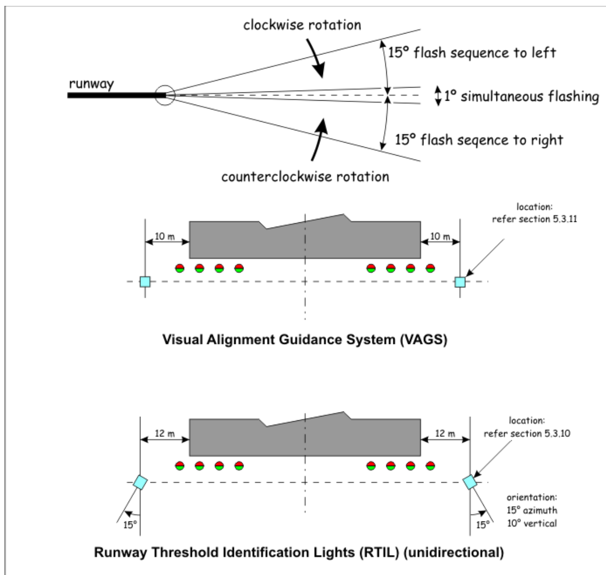
Figure 5-36: Configuration of VAGS and RTIL
