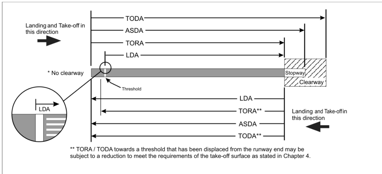
Figure 2-1: Illustration of declared distances
