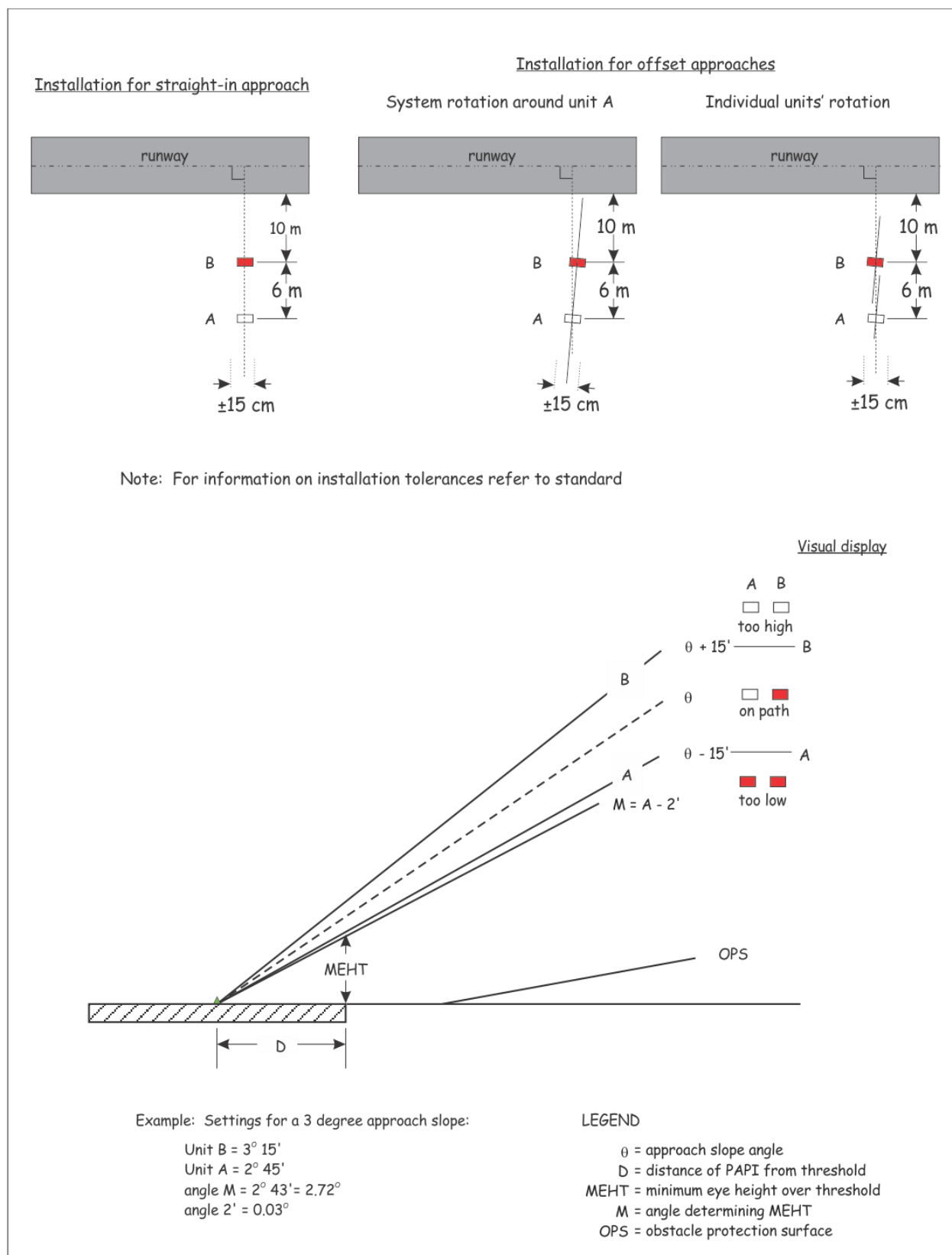
Figure 5-42: APAPI general arrangement
