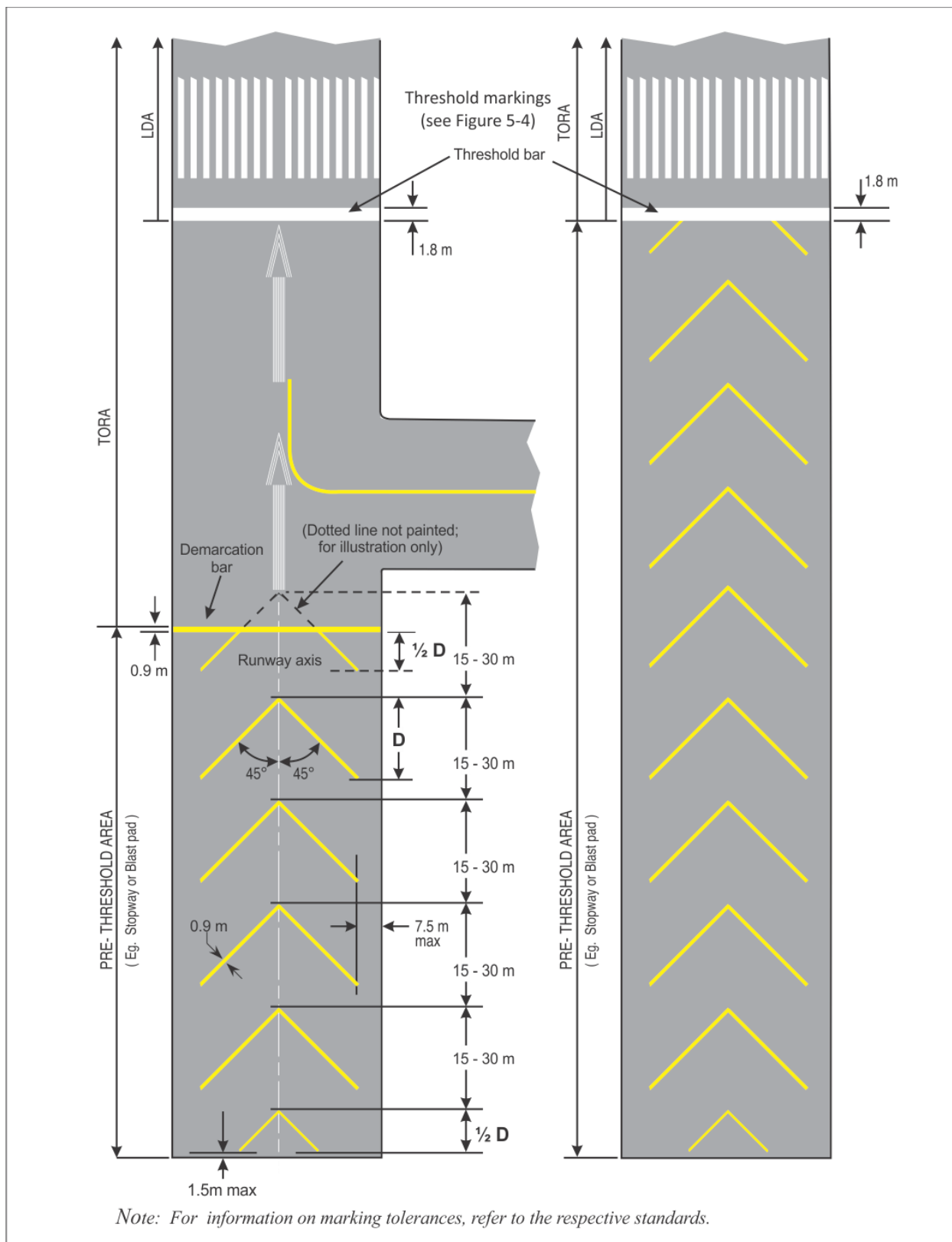
Figure 5-5: Chevrons, threshold bar and demarcation bar markings
