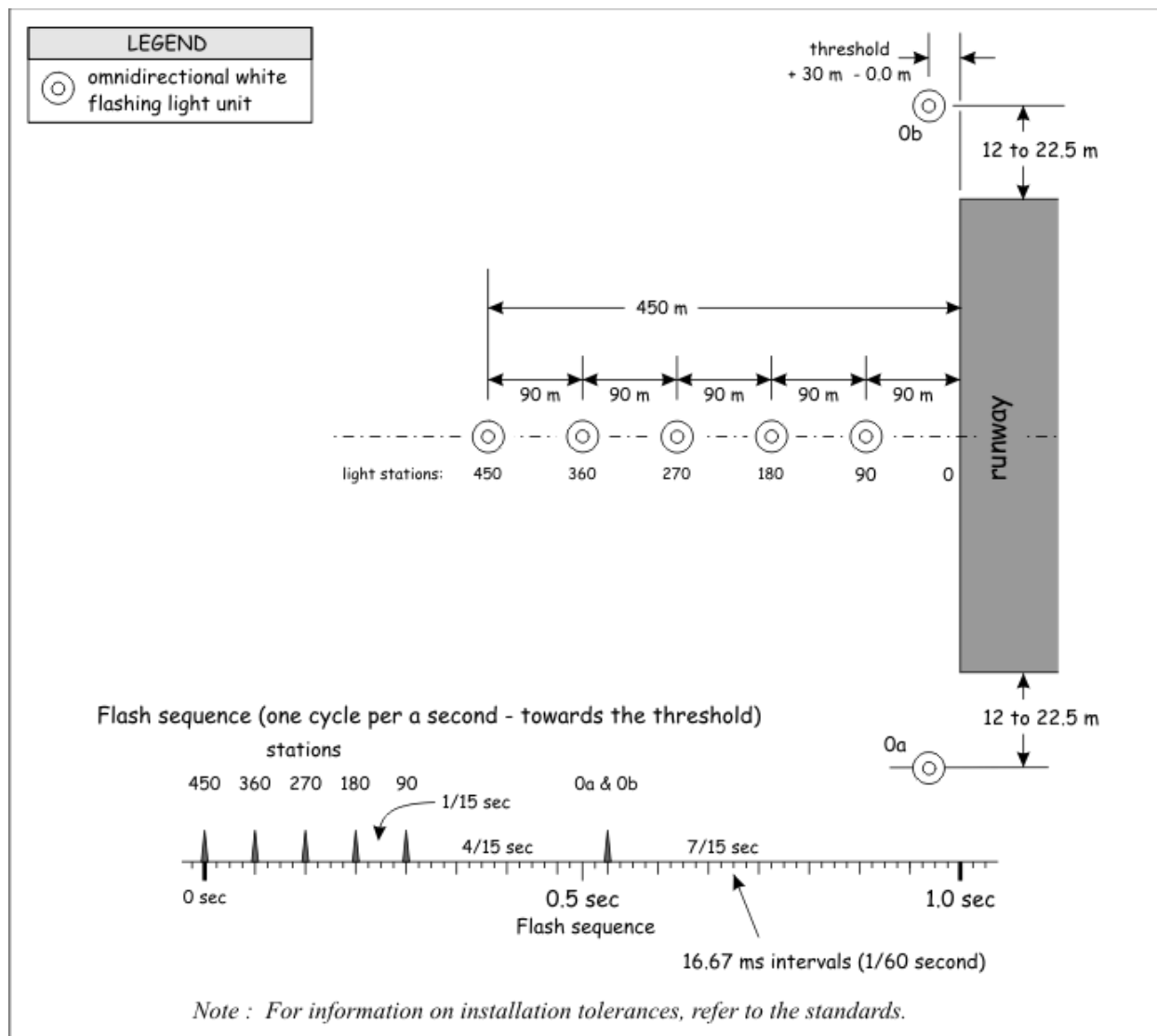
Figure 5-24: ODALS configuration
