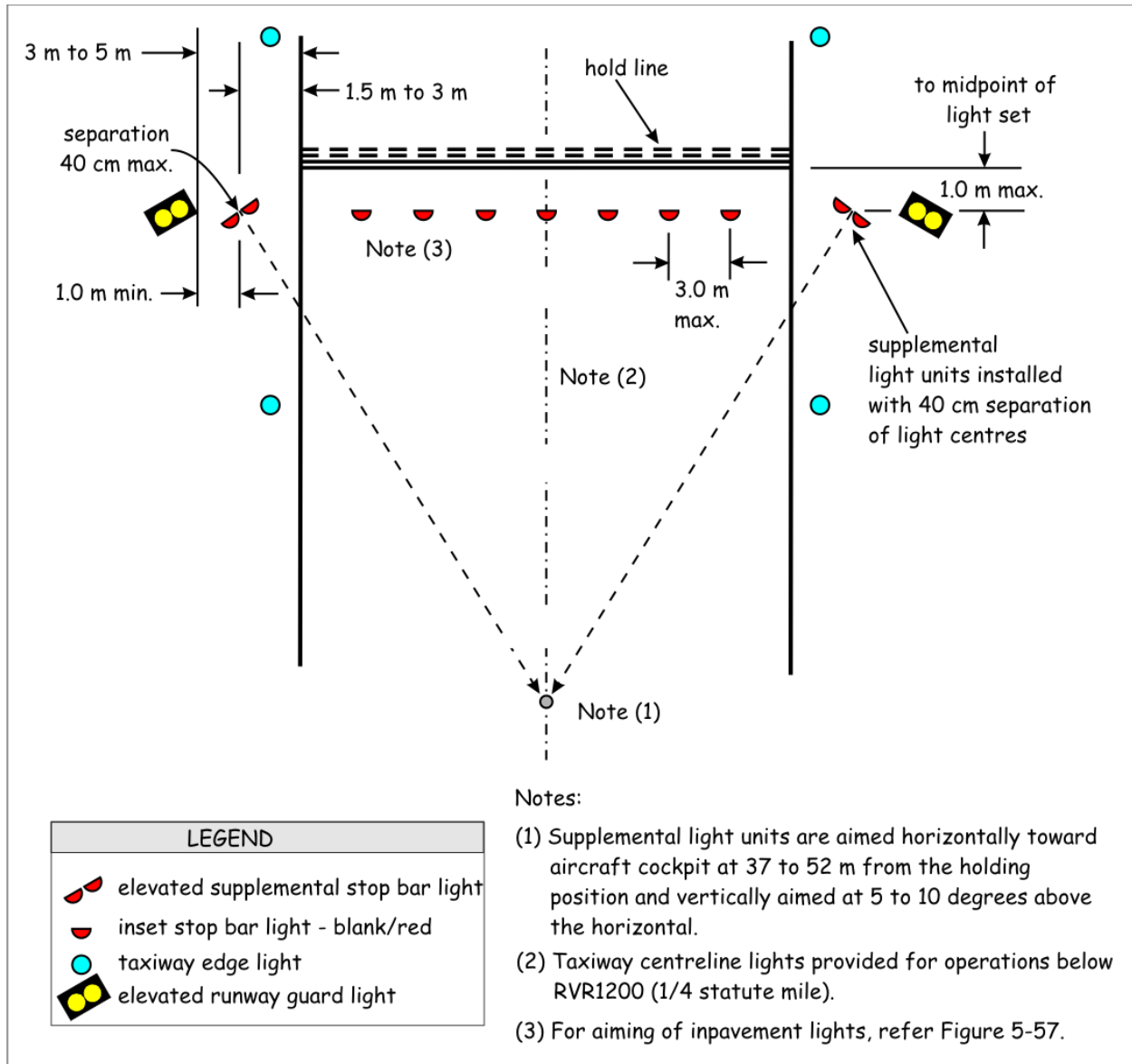
Figure 5-55: Stop bar lighting
