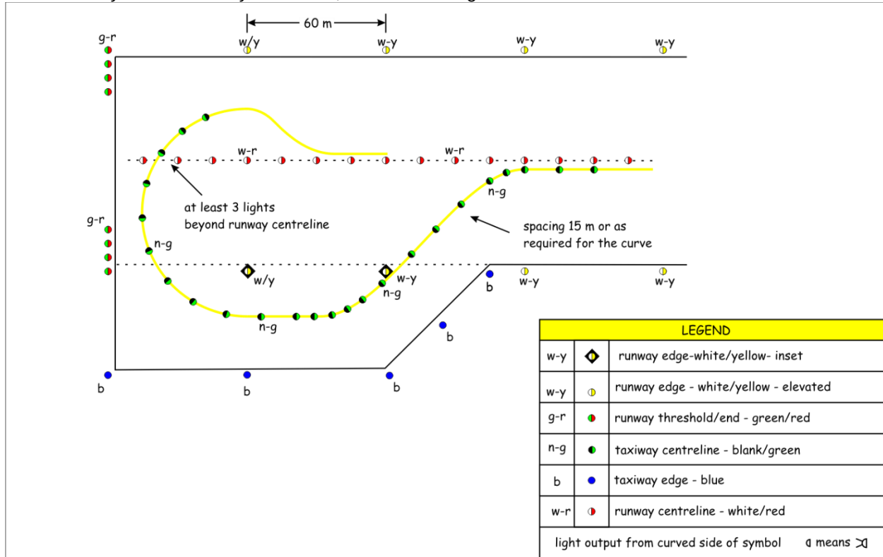
Figure 5-52: Runway turn pad lights
