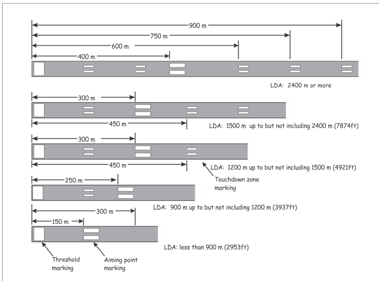
Figure 5-6(b): Aiming point and touchdown zone markings
