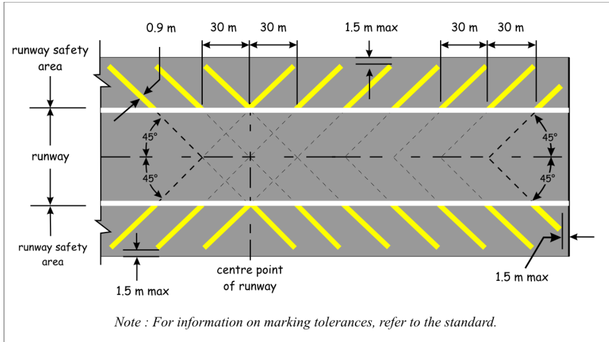
Figure 5-7: Runway side stripe and safety area markings
